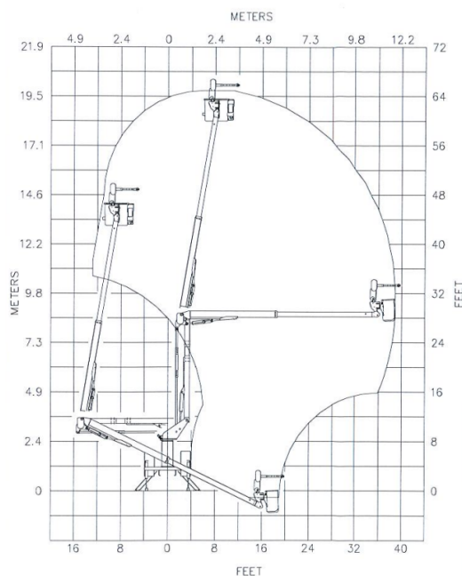
ECOTRUCK V-19.8 AT
