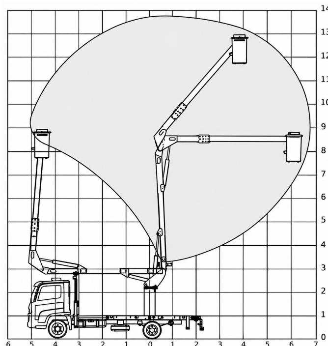
ECOTRUCK G-13.5 A
